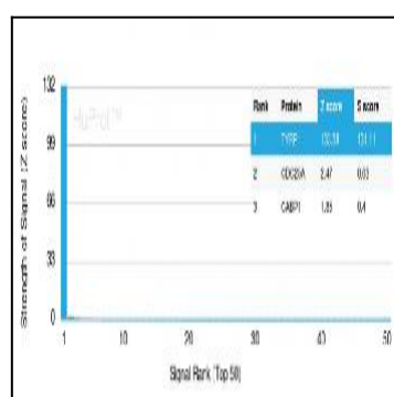
Fig. 3: Analysis of Protein Array containing more than 19,000 full-length human proteins using TYRP1-Monospecific Mouse Monoclonal Antibody (TYRP1/3284) Z- and S-Score: The Z-score represents the strength of a signal that a monoclonal antibody (Monoclonal Antibody) (in combination with a fluorescently-tagged anti-IgG secondary antibody) produces when binding to a particular protein on the HuProt™ array. Z-scores are described in units of standard deviations (SD's) above the mean value of all signals generated on that array. If targets on HuProt™ are arranged in descending order of the Z-score, the S-score is the difference (also in units of SD's) between the Z-score. S-score therefore represents the relative target specificity of a Monoclonal Antibody to its intended target. A Monoclonal Antibody is considered to specific to its intended target, if the Monoclonal Antibody has an S-score of at least 2.5. For example, if a Monoclonal Antibody binds to protein X with a Z-score of 43 and to protein Y with a Z-score of 14, then the S-score for the binding of that Monoclonal Antibody to protein X is equal to 29.
