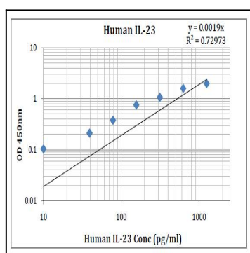
Fig-1: Human IL-23 Standard Curve.
