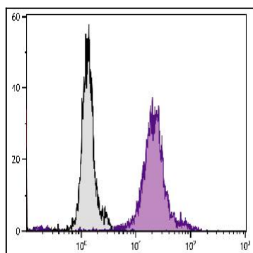
Figure 1: Human monocytes and granulocytes were stained with Mouse Anti-Human CD13-FITC .
