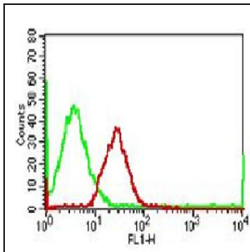
Figure-1: Cell surface flow analysis of hCD56 antibody on human PBMC (Monocytes gated) using 0.5 \mu g 10^6 cells. Green represents isotype control (ABEOMICS); red represents FITC conjugated anti-hCD56 antibody (10-7504F).
