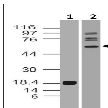
Figure-1: Western blot analysis of SMAD4. Anti- SMAD4 antibody (11-7581) was used at 0.1 \mu g/ml on (1) Recombinant and 2 \mu g/ml on (2) Hela lysates.
