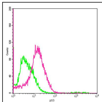
Figure-1 : Flow cytometric analysis of p53 Antibody (Clone: 6F2D3) on HEK293 at 2 \mu g for 1 \times 10^6 cells. Red histogram represents p53 Antibody (Clone: 6F2D3) and green histogram represents isotype control.
