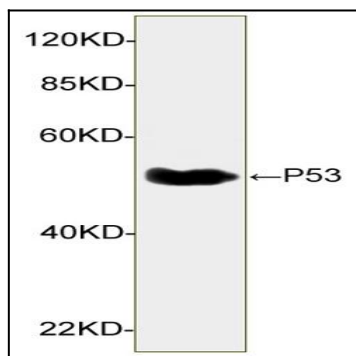
Figure-2 : Western blot analysis of p53 Antibody (Clone: 6F2D3) at 1 \mu g/ml on UV-treated HEK 293 cell lysates, IRDye 800 Conjugated Goat Anti-Mouse IgG was used as secondary Antibody.
