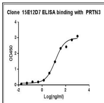
Figure-1 : ELISA binding of Human PRTN3 Antibody (Clone: 15E12D7) with Human PRTN3 recombinant protein, Coating antigen: PRTN3 at 1 µg/ml, PRTN3 antibody dilution start from 1000 ng/ml, EC50= 13.17 ng/ml.
