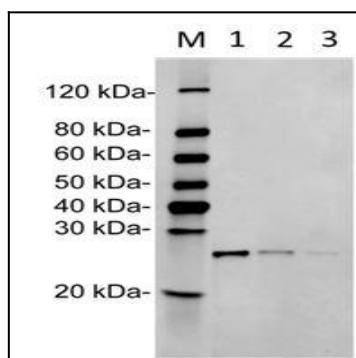
Figure-2 : Western Blot analysis of PRTN3 Antibody (Clone: 15E12D7) at 1 µg/ml on Human PRTN3 recombinant protein (1-3: 50 ng, 10 ng & 5 ng), IRDye 800 conjugated Goat anti-Mouse IgG was used as Secondary Antibody at 0.125 µg/ml.
