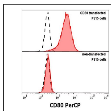
Figure 1: Anti-human CD80 PerCP antibody (clone MEM-233) specificity verification by flow cytometry
