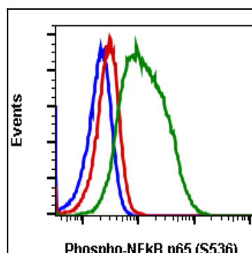
Fig-1: Flow cytometric analysis of HeLa cells unstained and untreated as negative control (blue) or stained and untreated (red) or stained and treated with TNFα plus CalA (green) using phospho-NFkB p65 (Ser536) antibody NFKBP65S536-B7 at 0.05 µg/mL.
