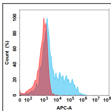
Figure 1. Flow cytometry analysis with 15 \mu g/mL Anti-OSMR (vixarelimab biosimilar) mAb on Expi293 cells transfected with Human OSMR protein (Blue histogram) or Expi293 transfected with irrelevant protein (Red histogram).
