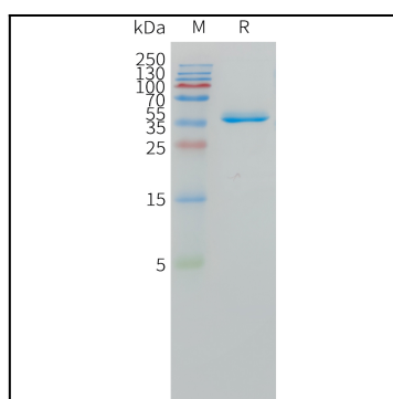
Figure 1. Human DLL3 (428-492) Protein, hFc Tag on SDS-PAGE under reducing condition.
