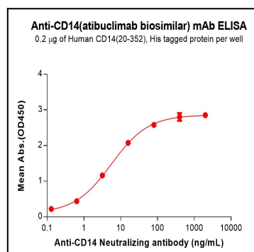
Figure 1. ELISA plate pre-coated by 2 µg/mL (100 µL/well) Human CD14(20-352) Protein, His Tag can Anti-CD14(atibuclimab biosimilar) mAb in a linear range of 0.64-80 ng/mL.
