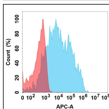
Figure 2. Flow cytometry analysis with 15 µg/mL Anti-CD14(atibuclimab biosimilar) mAb on Expi293 cells transfected with Human CD14 protein (Blue histogram) or Expi293 transfected with irrelevant protein (Red histogram).
