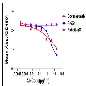
Figure 1. Elisa plates were pre-coated with His Tagged Feline IL31 protein (0.1µg/per well). 1µg of Feline IL31RA, mFc Tagged protein and serial dilutions of anti-Feline IL31 monoclonal antibody were added, and Goat anti Mouse IgG(Horseradish Peroxidase Conjugate) was used as the secondary antibody. From the above data, the biosimilar(Red) and clone 6G1(Blue) have good competitive activity, and Rabbit IgG(Purple) was used as the Isotype Control.
