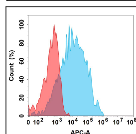
Figure 2. Flow cytometry analysis with 1µg/mL Anti-FGFR3 (vofatamab biosimilar) mAb (12-90012) on Expi293 cells transfected with Human FGFR3 protein (Blue histogram) or Expi293 transfected with irrelevant protein (Red histogram).
