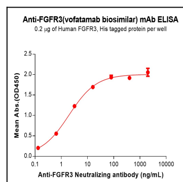
Figure 1. ELISA plate pre-coated by 2 µg/mL (100 µL/well) Human FGFR3 Protein, His Tag can bind Anti-FGFR3 (vofatamab biosimilar) mAb (12-90012) in a linear range of 0.13–16 ng/mL.
