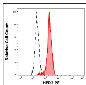
Figure 1: Separation of MCF-7 cells stained using anti-human HER3 (H3Mab-17) PE antibody (concentration in sample 0.56 µg/ml, red-filled) from MCF-7 cells stained using mouse IgG2a isotype control (MOPC-173) PE antibody (concentration in sample 0.56 µg/ml, same as HER3 PE concentration, black-dashed) in flow cytometry analysis (surface staining).
