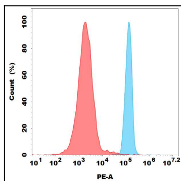
Figure 1. Flow cytometry analysis with 1 \mu l/test PE-conjugated Anti-5T4 (H8 biosimilar) mAb on HEK293 cells (Blue histogram) or Jurkat cells (Red histogram).
