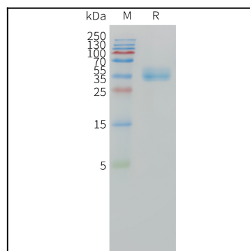
Figure 1. Human CA12 Protein, His Tag on SDS-PAGE under reducing condition.
