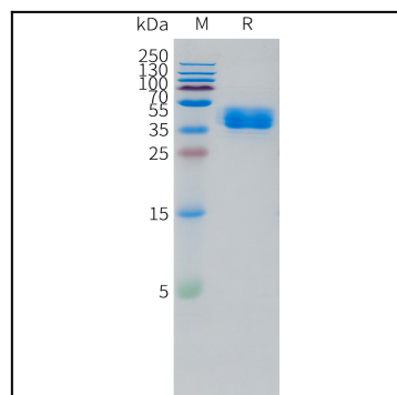
Figure 1. Human TRHR Protein, hFc Tag on SDS-PAGE under reducing condition.
