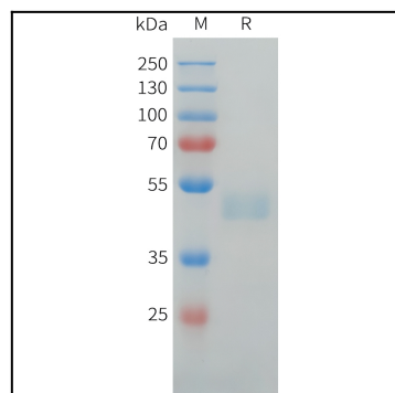
Figure 1. Human CDH17(129-244) Protein, hFc Tag on SDS-PAGE under reducing condition.
