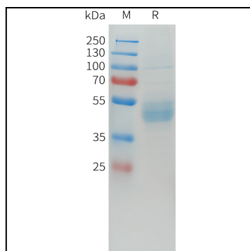
Figure 1. Human CDH17(341-449) Protein, hFc Tag on SDS-PAGE under reducing condition.
