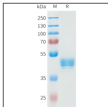
Figure 1. Human CDH3(108-215) Protein, hFc Tag on SDS-PAGE under reducing condition.
