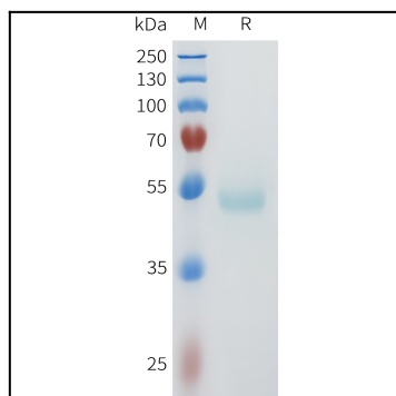
Figure 1. Human Nectin-4(238-349) Protein, hFc Tag on SDS-PAGE under reducing condition.
