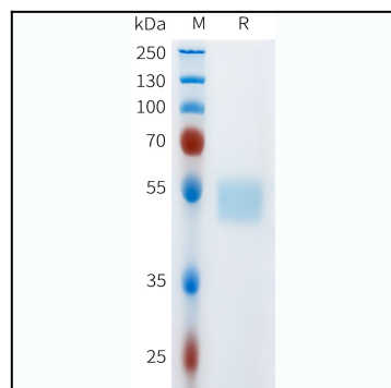
Figure 1. Human CD117(309-412) Protein, hFc Tag on SDS-PAGE under reducing condition.
