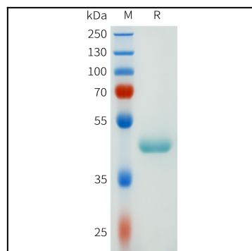
Figure 1. Human CSF1R(198-298) Protein, hFc Tag on SDS-PAGE under reducing condition.
