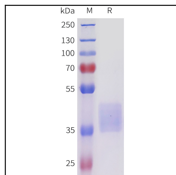
Figure 1. Human ACVR2B(98-134) Protein, mFc Tag on SDS-PAGE under reducing condition.
