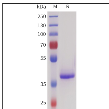
Figure 1. Human SEZ6(355-415) Protein, hFc Tag on SDS-PAGE under reducing condition.
