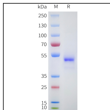
Figure 1. Human LGR5(447-561) Protein, hFc Tag on SDS-PAGE under reducing condition.
