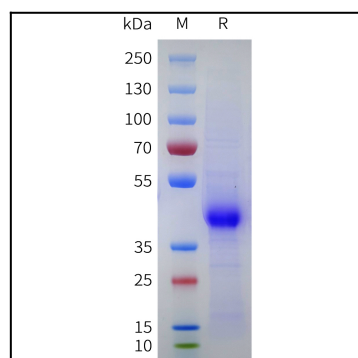
Figure 1. Human CD43 Protein, His Tag on SDS-PAGE under reducing condition.
