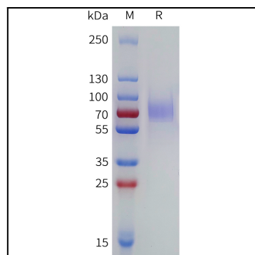
Figure 1. Human LILRB1 Protein, His Tag on SDS-PAGE under reducing condition.
