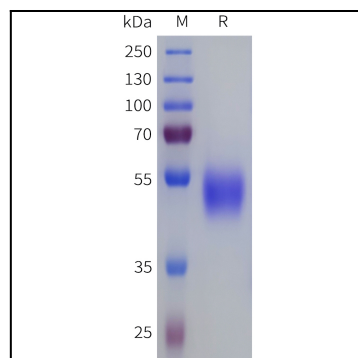
Figure 1. Human SSTR3 Protein, hFc Tag on SDS-PAGE under reducing condition.
