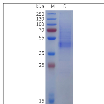
Figure 1. Human DCN(17-359) Protein, His Tag on SDS-PAGE under reducing condition.
