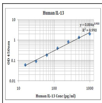
Fig-1: Human IL-13 Standard Curve
